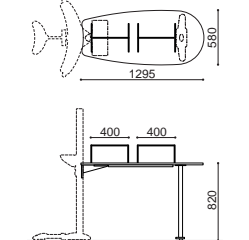
27 Single shelf model JJA-105W-W9 Capacity: 0.4f/m x 4 Load capacity: 60kg
