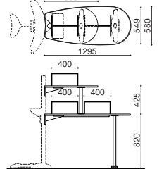
25 2-shelf model (with small upper shelf) JJA-135WS-W9 Capacity: 0.4f/m x 6 Load capacity: 60kg (lower shelf), 30kg (upper shelf)
