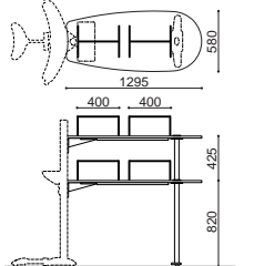
26 2-shelf model JJA-135WW-W9 Capacity: 0.4f/m x 8 Load capacity: 30kg for upper step, 60kg for lower step
